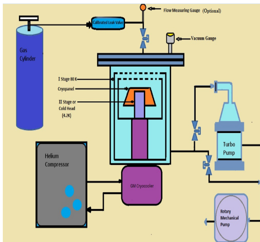
Fig. 1 Block diagram of Experimental setup
