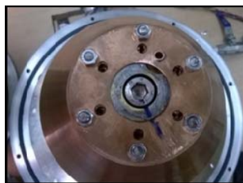
Fig. 5 Bare panel with adhesive mounted on cryocooler
