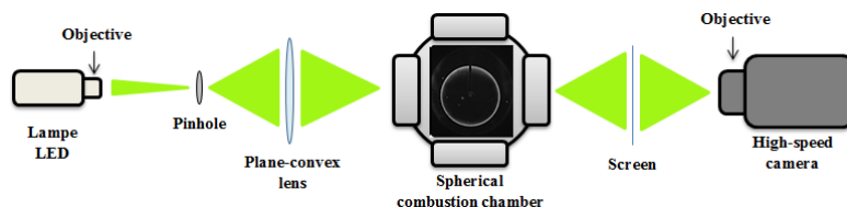
Fig. 1 Scheme of the experimental setup
