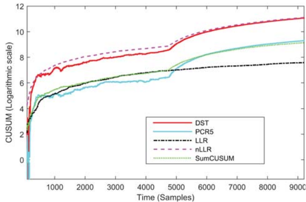
Fig. 9 CUSUM results for USRP data
