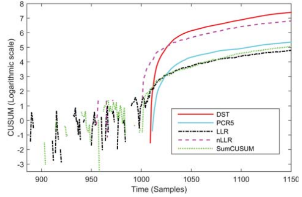
Fig. 5 CUSUM results for test data when distributions are known
