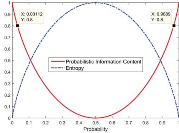
Fig. 4 Entropy and Probabilistic information content
