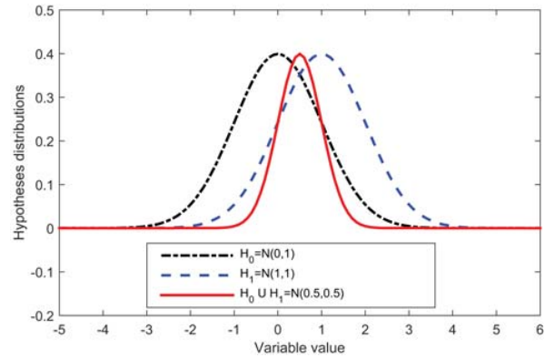
Fig. 2 Hypotheses distributions including null, alternative and uncertainty
