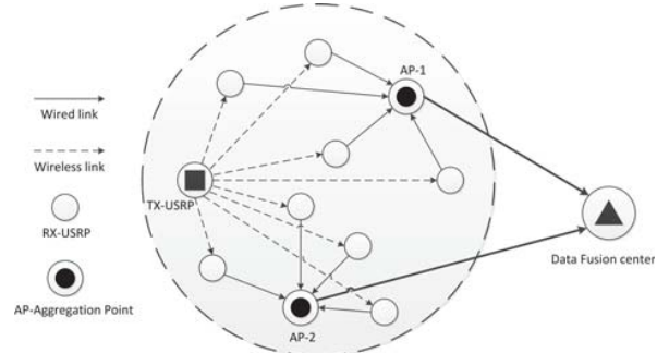
Fig. 8 Cooperative spectrum sensing setup
