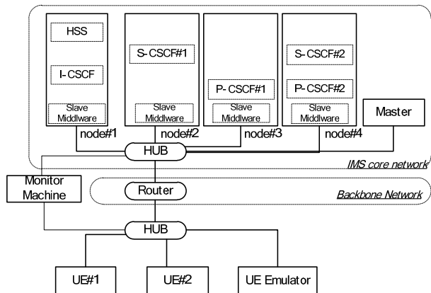
Fig. 7 Experimental Network Configuration
