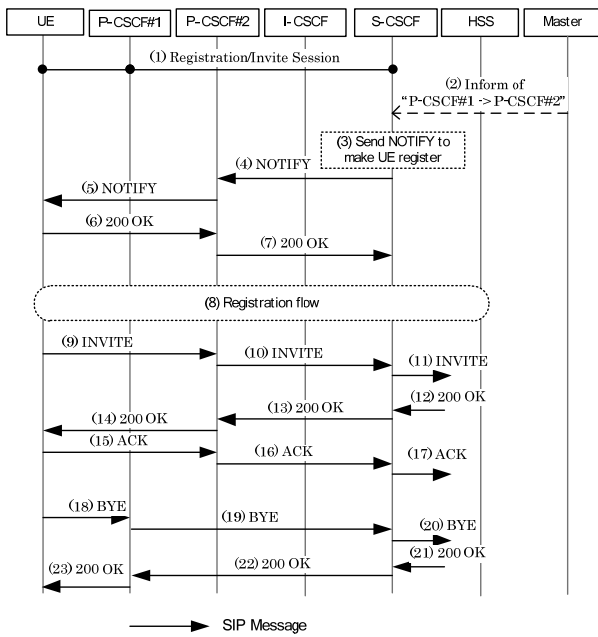
Fig. 5 P-CSCF Change Flow
