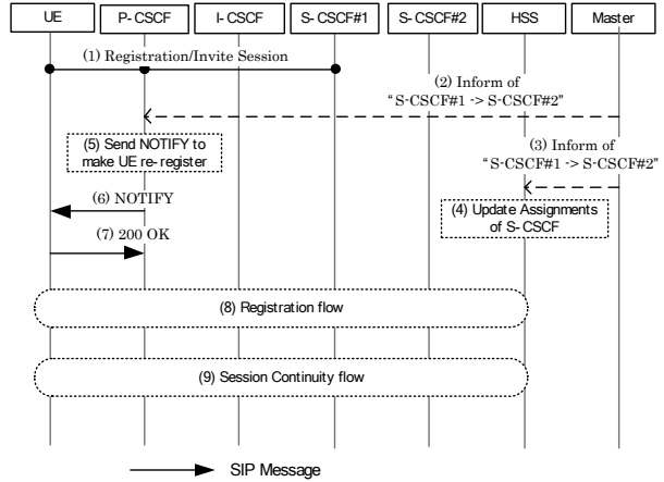
Fig. 6 S-CSCF Change Flow
