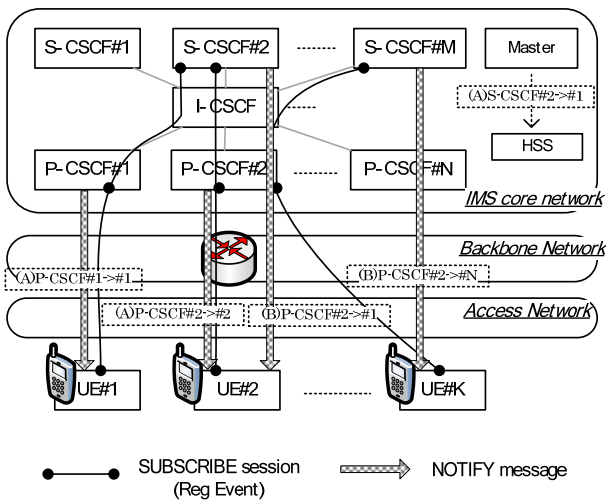
Fig. 3 Overview of Notification Method
