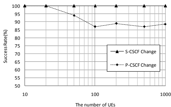
Fig. 12 Success Rate of CSCF Change
