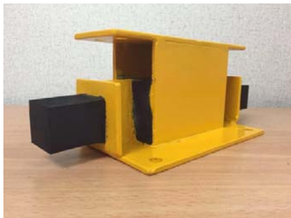
Fig. 2 The hybrid viscoelastic energy dissipation device
