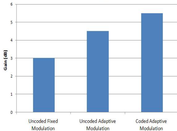
Illustration of Coding Gain in dB
