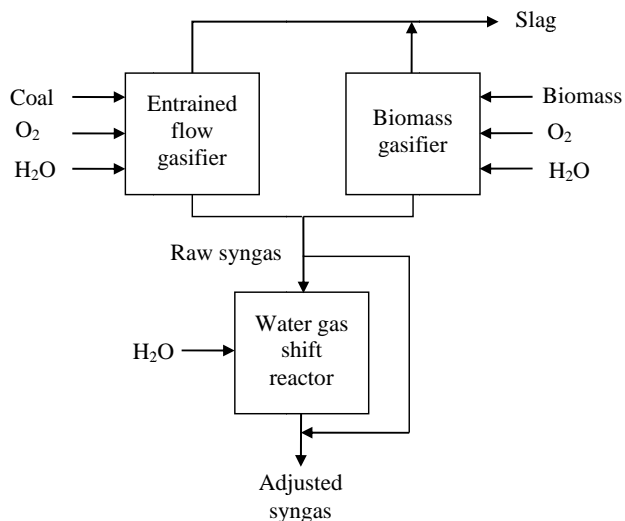
Fig. 2 Schematic diagram for independent co-gasification process
