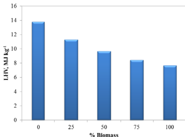
Fig. 5 Heating values for the produced raw syngas
