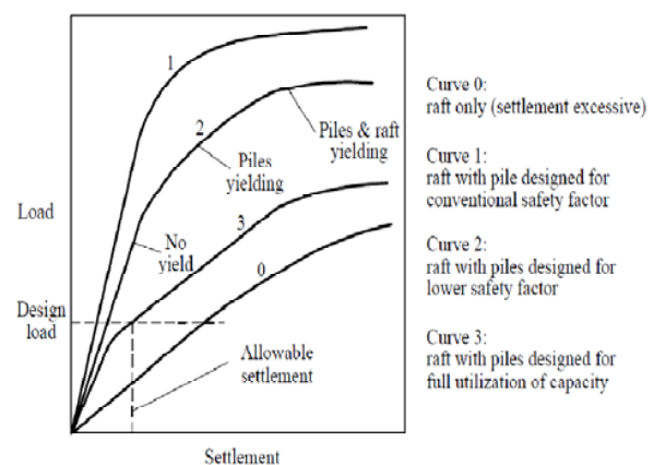
Fig. 1 Load settlement curves for piled rafts [1]
