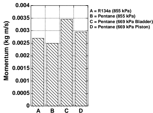
Fig. 10 Momentum values at the 10 ms pulse-width
