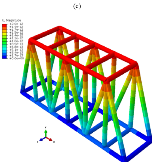
Fig. 7 Displacement in trusses a) Hawe, b) K, c) Pratt and d) Warren under cyclic load
