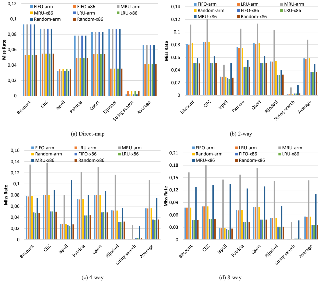
Fig. 2 The effect of different replacement policies on performance of the cache (cache size: 16 KB)
