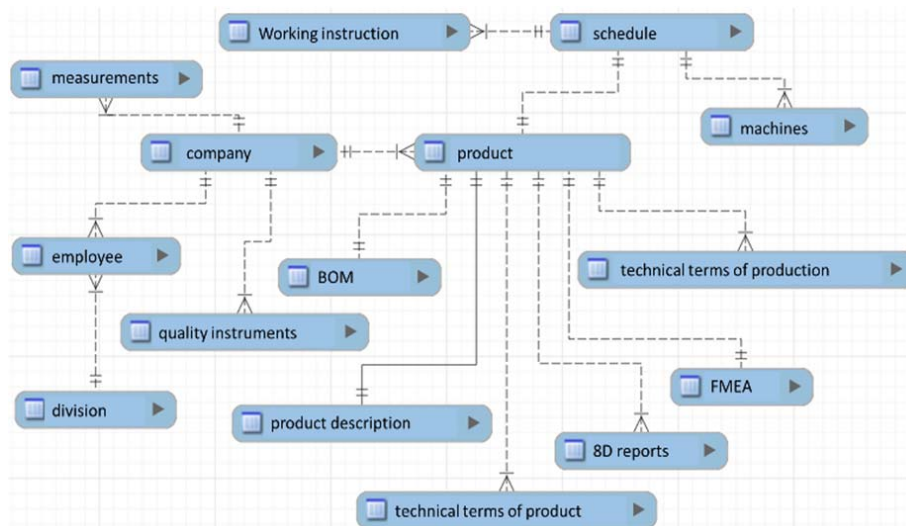
Fig. 4 Meta model as basis for content evaluation
