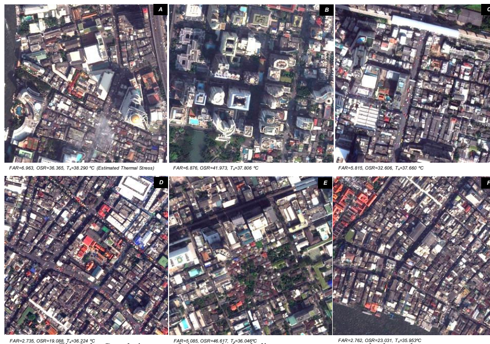
Fig. 9 the Google images of six sample local climate zones are extremely thermal stress
