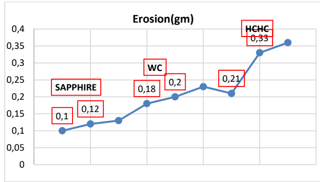
Fig. 26 Erosion graph of different nozzles
