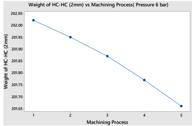
Fig. 20 Weight loss of HC-HC nozzle of 2 mm dia under pressure 6 bar
