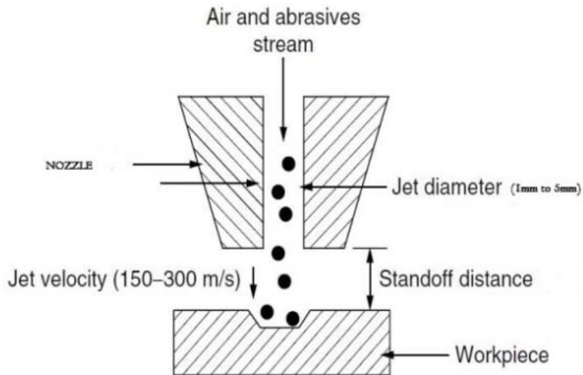
Fig. 5 Working of nozzle
