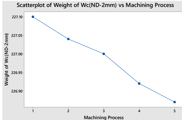
Fig. 14 Weight loss of WC nozzle of 2 mm dia under pressure 6 bar
