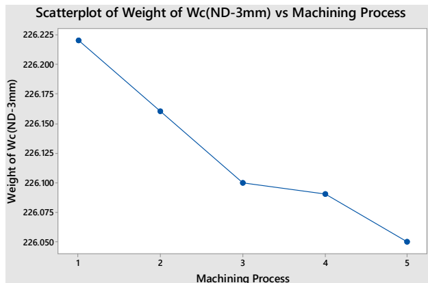
Fig. 16 Weight loss of WC nozzle of 3 mm dia under pressure 6 bar
