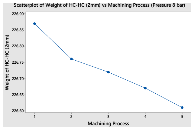
Fig. 21 Weight loss of HC-HC nozzle of 2 mm dia under pressure 8 bar
