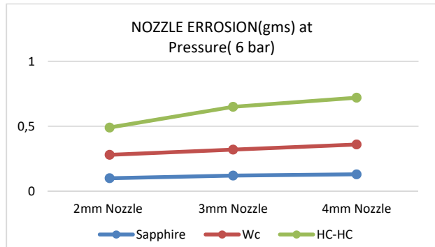
Fig. 27 Nozzle erosion vs pressure (6 bar)
