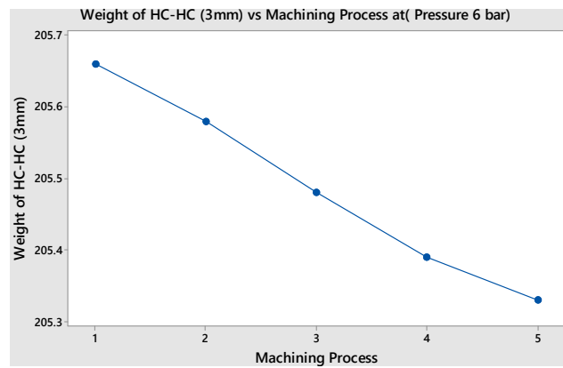
Fig. 22 Weight loss of HC-HC nozzle of 3 mm dia under pressure 6 bar
