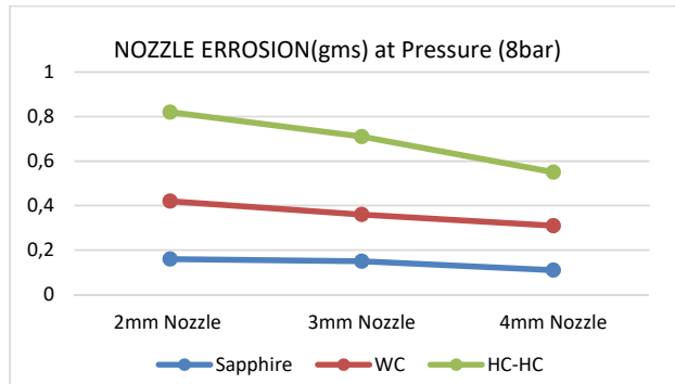
Fig. 28 Nozzle erosion vs pressure (8 bar)
