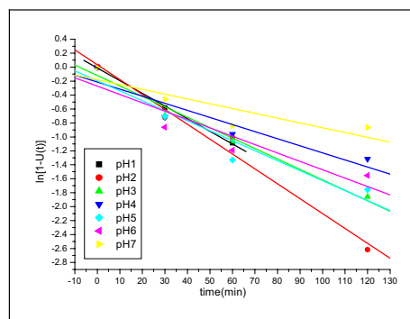
Fig. 3 1 st order reversible reaction
