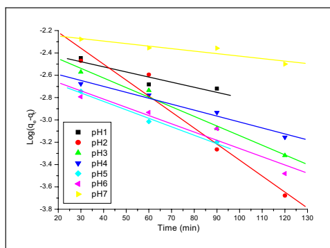
Fig. 2 Lagergren's plot
