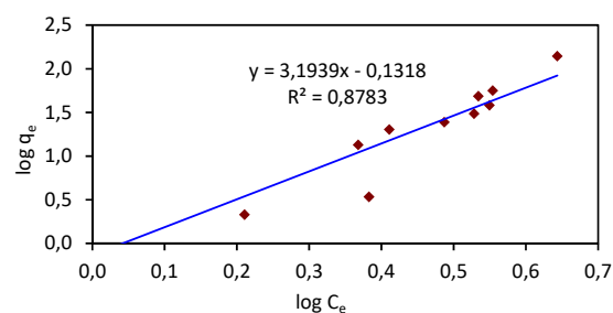
Fig. 8 Freundlich isotherm plots for the removal of \text{Pb}^{2+} by activated carbon using \text{H}_3\text{PO}_4 60% solution and carbonation temperature of 600^\circ\text{C} (temperature = 26^\circ\text{C} , contact time = 180 min)
