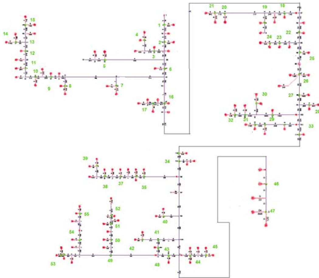
Fig. 1 Single-line diagram of Al-Qatrah transmission line
