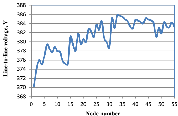
Fig. 4 Average line-to-line voltages of the load nodes as expected in the year 2020 with a STATCOM installed at different nodes
