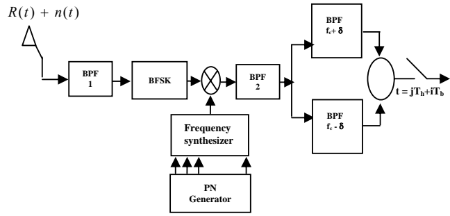
Fig. 1. Block diagram of the SFH/BFSK receiver system.
