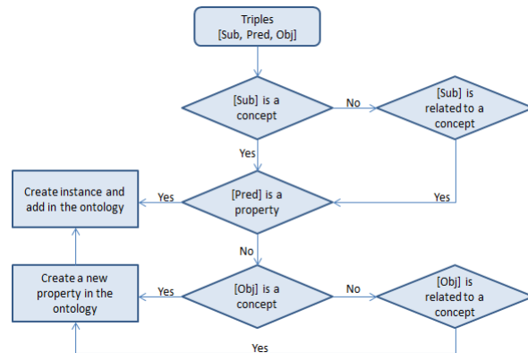
Fig. 3 Validation algorithm
