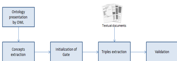
Fig. 2 Extraction algorithm from textual documents
