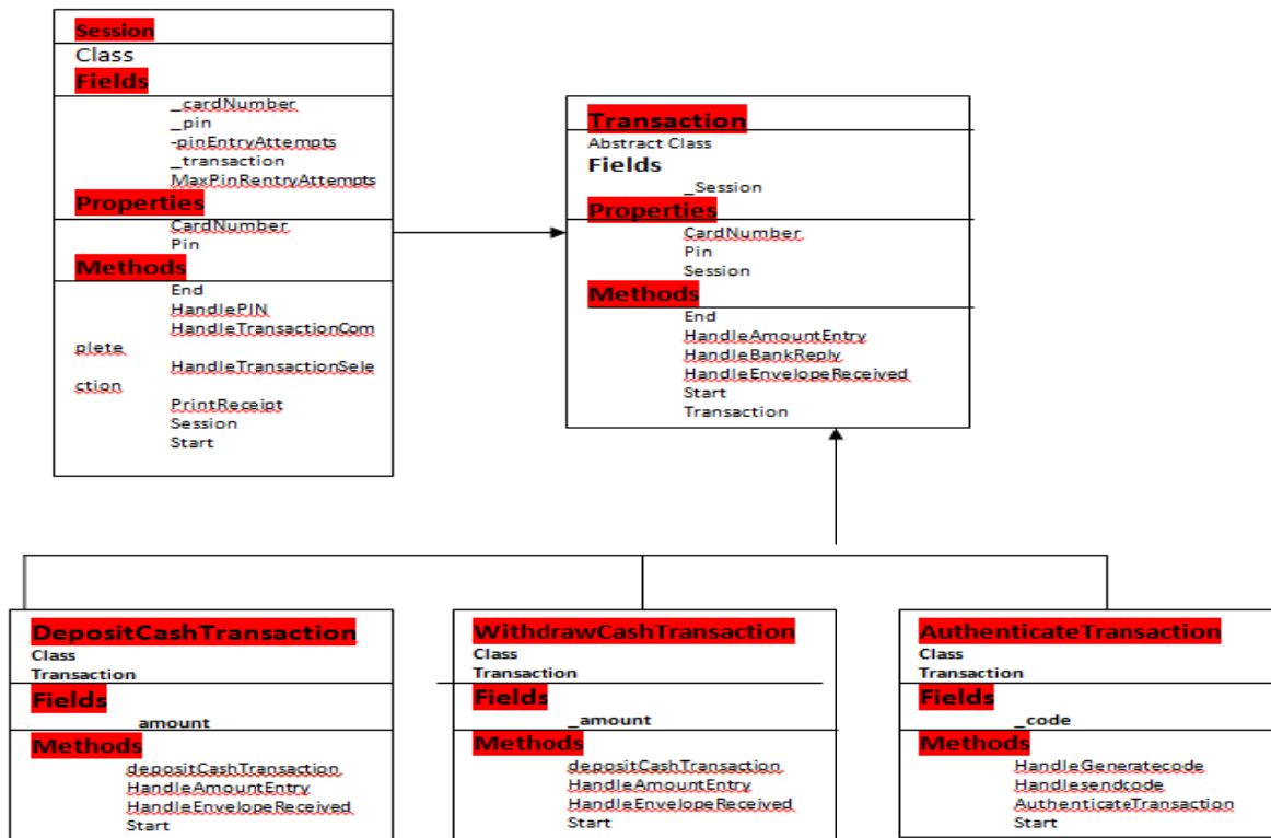
Fig. 2 Class Diagram
