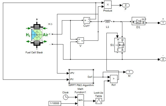
Fig. 5 PEMFC with boost converter
