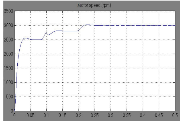
Fig. 8 Motor speed waveform
