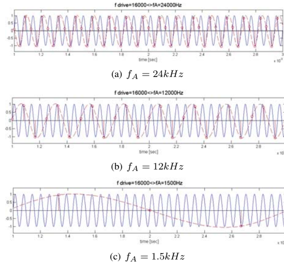
Fig. 3. Time domain of the appearing aliasing signals after under-sampling the drive signal with different sampling frequencies
