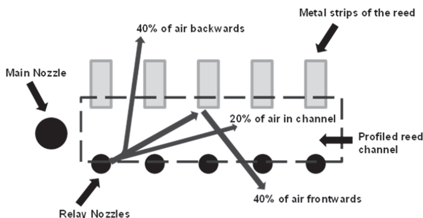
Fig. 6 Schematic of weft passage region
