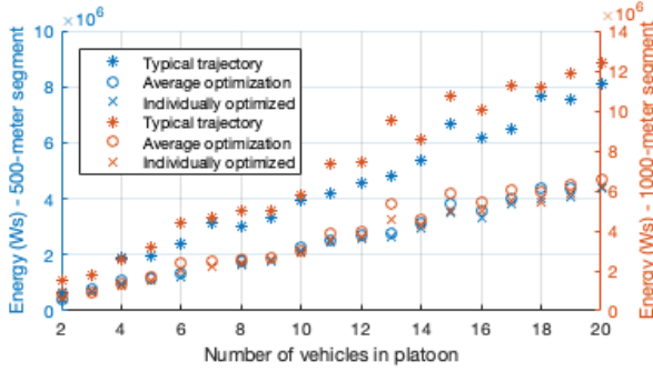
Fig. 4 Total energy spent by vehicles in a platoon for a 500m segment.
