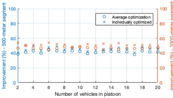
Fig. 5 Improvement in total energy spent by vehicles in a platoon for a 500m segment.
