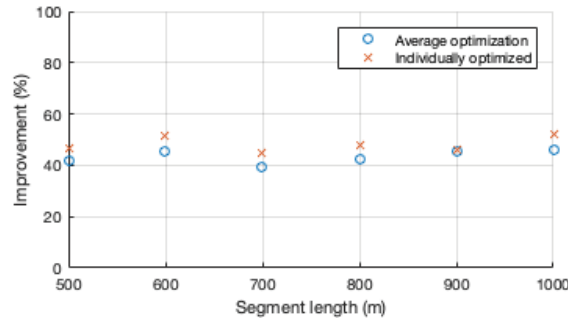
Fig. 7 Improvement in total energy spent by 10 randomly chosen vehicles in a platoon for different segment lengths with an average speed of 10 m/s.
