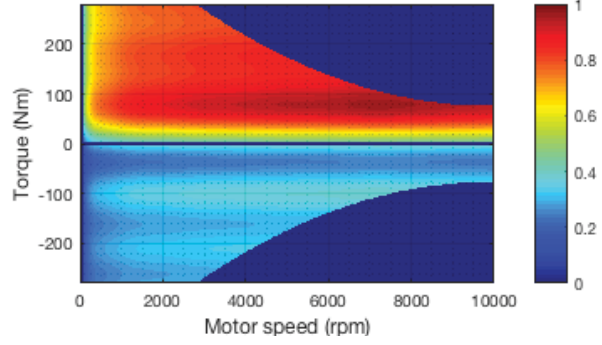
Fig. 1 Typical characterization of efficiencies.
