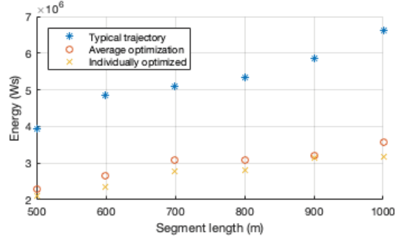
Fig. 6 Total energy spent by 10 randomly chosen vehicles in a platoon for different segment lengths with an average speed of 10 m/s.
