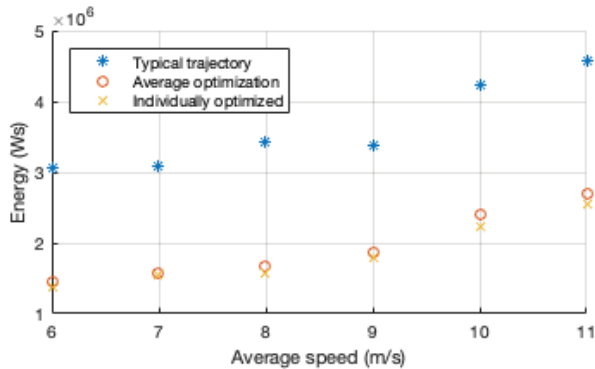
Fig. 8 Total energy spent by 10 randomly chosen vehicles in a platoon for different average speeds in a 500-meter segment.
