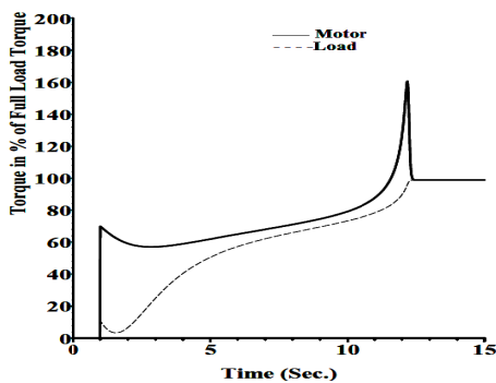
Fig. 6 Motor and Load torques during motor starting
