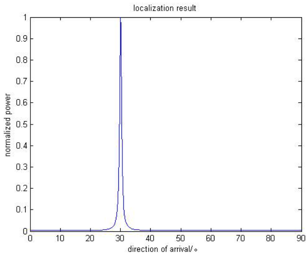
Fig. 4 Normalized power
