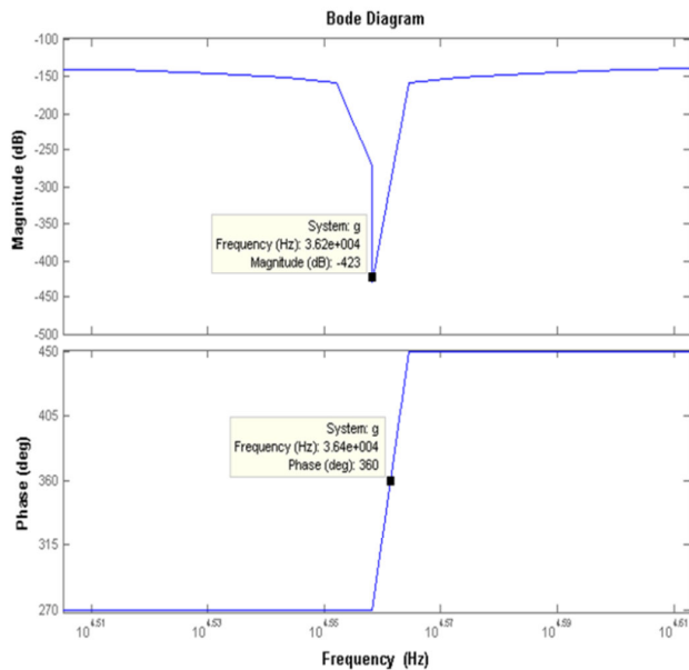
Fig. 5 Bode plot for the electrical model of the microcantilever
