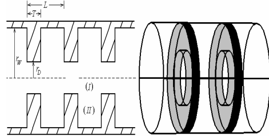
Fig.1 Schematic of a circular waveguide loaded with annular metal discs showing the structure regions (I and II) and disc parameters.
