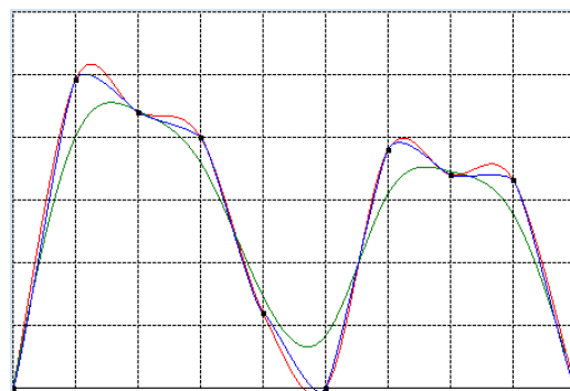
Fig. 2 comparing interpolation curves. Black points are control points. Red curve is Catmull-rom interpolation, green curve is cubic B-spline and blue curve is proposed interpolation curve
