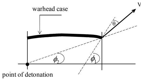
Fig. 2 Spray angle of fragment
