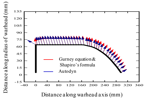
Fig. 9 Comparison of velocity vectors of fragments of warhead obtained from analytical calculation and numerical analysis case2
