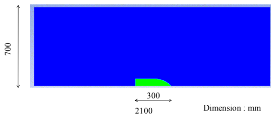
Fig. 7 Domain of air, explosive, and warhead casing in FE analysis
