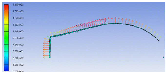
Fig. 15 Velocity vectors obtained from Autodyn at time = 0.045 msec
