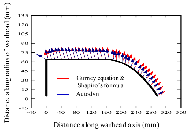
Fig. 13 Comparison of velocity vectors of fragments of warhead obtained from analytical calculation and numerical analysis case6
