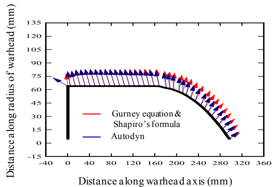
Fig. 11 Comparison of velocity vectors of fragments of warhead obtained from analytical calculation and numerical analysis case4
