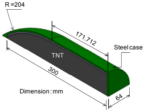
Fig. 1 Shape and dimension of a dummy warhead
