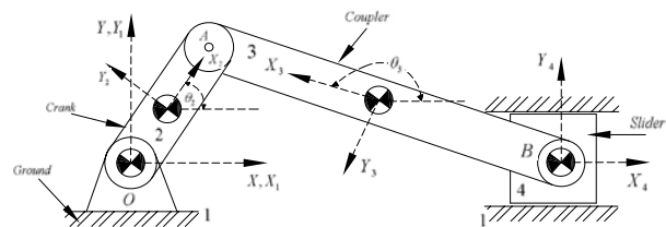
Fig. 4. Slider-crank mechanism
