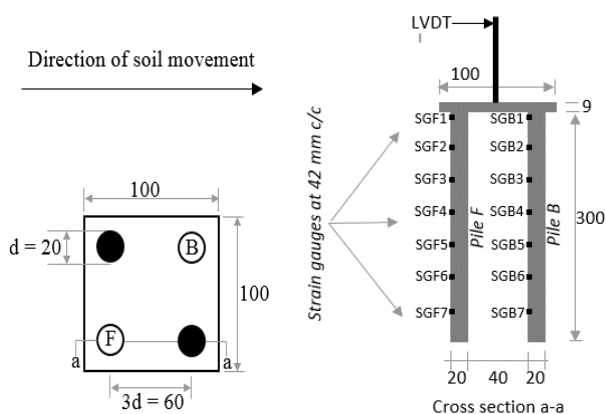
Fig. 5 Details of model piles and cap
