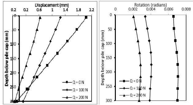
(a) Deflection of the front pile (b) Rotation of the front pile
