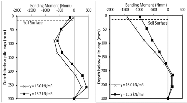
(a) Pile F (b) Pile B Fig. 6 Moment profiles of piles at \Delta B = 20 mm
