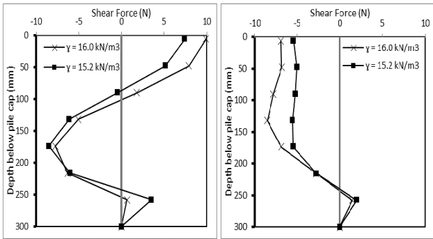
(a) Pile F (b) Pile B Fig. 7 Shear force profiles of piles at \Delta B = 20 mm
