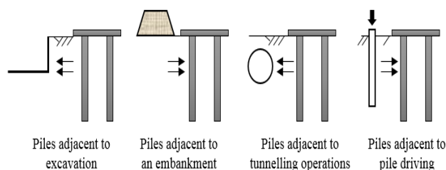
Fig. 1 Examples of passive piles
