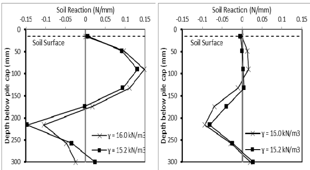
(a) Pile F (b) Pile B Fig. 8 Soil reaction profiles of piles at \Delta B = 20 mm
