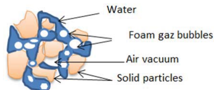
Fig. 4 Structure of soil-foam matrix
