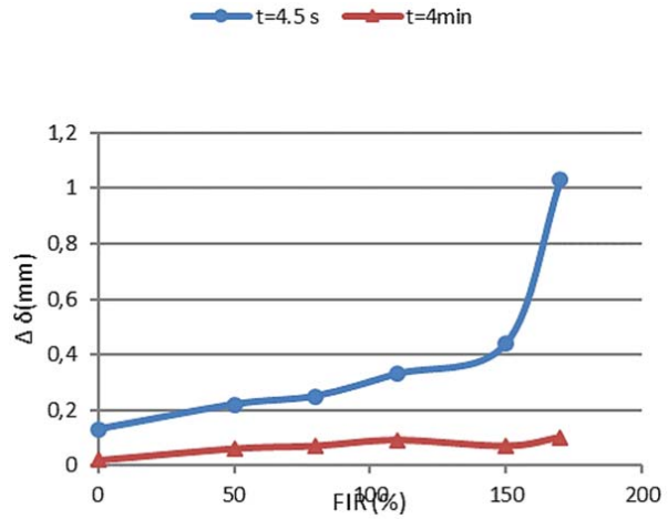
Fig. 8 Effect of loading on the foam
