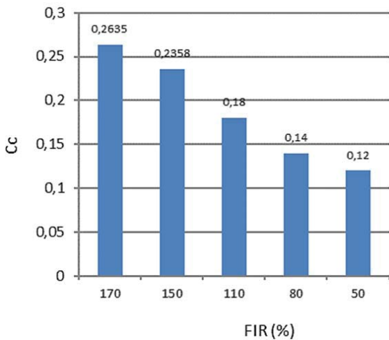
Fig. 7 Compression index variation depending on the FIR
