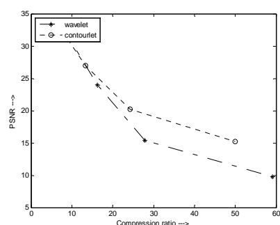
Fig. 10 Comparison of CR vs. PSNR between Wavelet and Contourlet transform for test image 8
