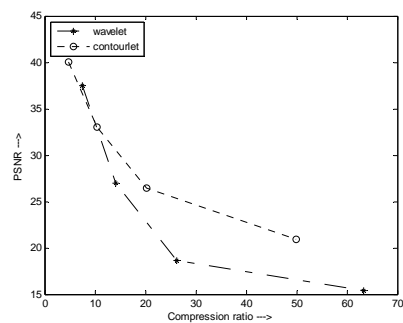
Fig. 9 Comparison of CR vs. PSNR between Wavelet and Contourlet transform for test image 7
