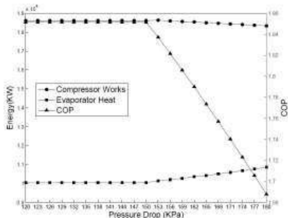
Fig.10. Variation of COP and Evaporator Heat and Compressor Works (kW) with the change in V-3 Pressure Drop.
