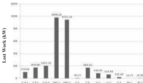
Fig. 4. Lost work of refrigeration cycle components.
