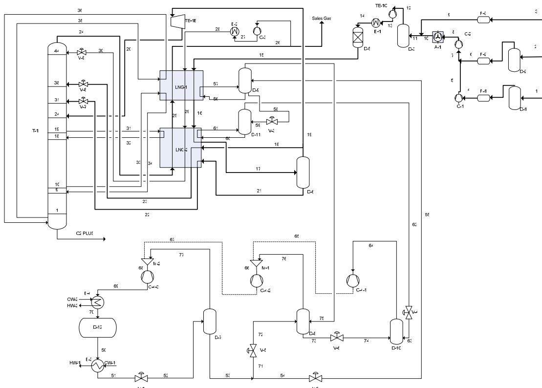
Fig.1. Propane refrigeration cycle used in C_2^+ recovery plant (CRP).
