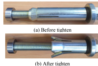
Fig. 2 Extended Hollobolt
