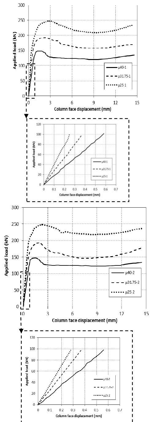
Fig. 5 Applied load versus the column face displacement curves for \mu 40, \mu 31.75 and \mu 25
