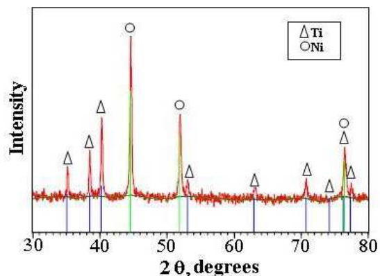
Fig. 2 XRD pattern of the mechanically alloying Ni-Ti powders
