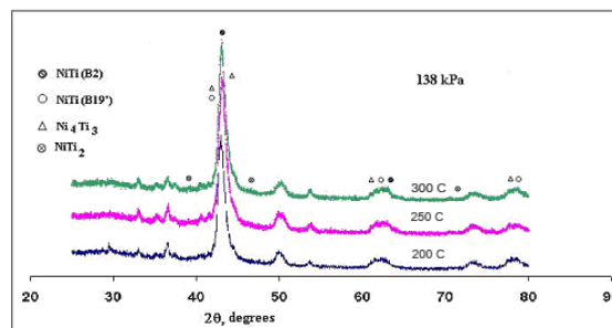
Fig. 3 XRD patterns of the SHS-synthesized porous NiTi SMAs at a chamber pressure of 138 kPa with different preheating temperatures of 200°C, 250 °C and 300°C
