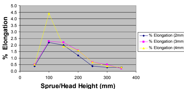
Fig. 7 Percent elongation of TWDI castings with sprue height
