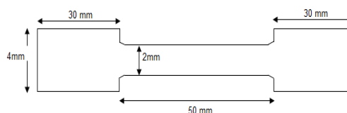
Fig. 4 Dimension for tensile test sample
