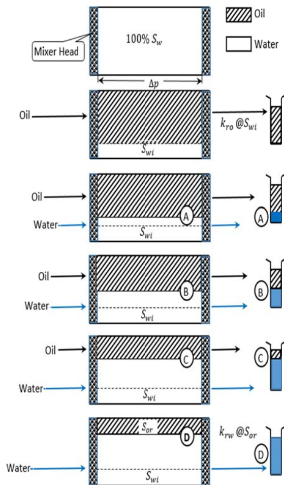
Fig. 1 Oil and water flow under various saturation [2], [3]
