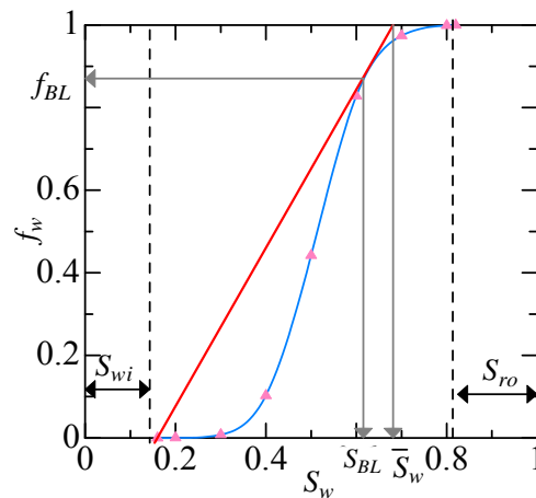
Fig. 5 Fractional flow
