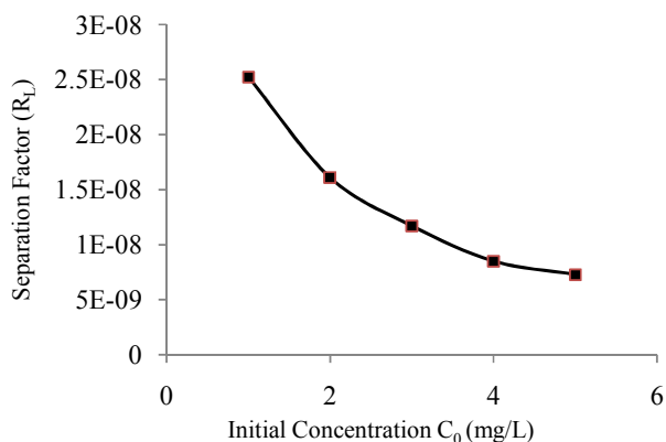
Fig. 12 showing the separation factor R_L vs initial cobalt concentrations. The R_L values were found to be between 0 and 1 using Langmuir constant K_a ( L.mg^{-1} )
