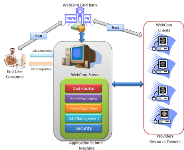
Fig. 7 High Level View of the Economic Setup
