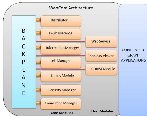
Fig. 1 WebCom architecture
