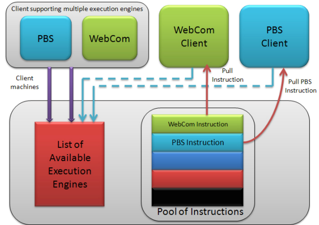
Fig. 3 The WebCom Distributor Module.
