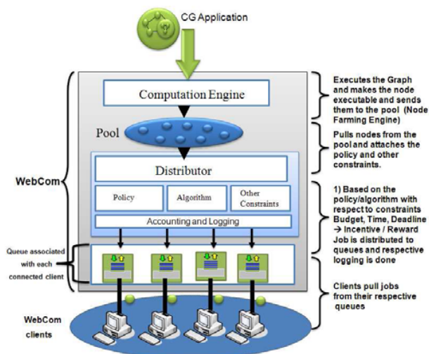
Fig. 2 Reward-Based Distributor in WebCom
