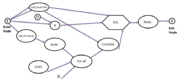
Fig. 6 Mandelbrot Graph Application
