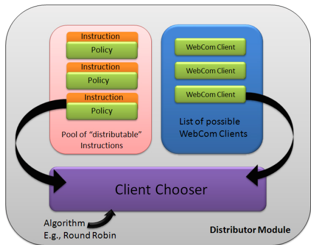
Fig. 4 Choosing appropriate clients within WebCom
