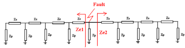
Fig. 3 Fault at the transmission pole
