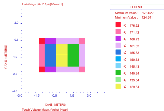
Fig. 11 Touch Voltage computation under 227V EPR
