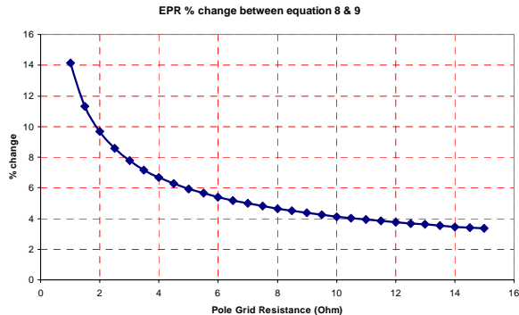
Fig. 5 EPR percentage change when using equation 9
