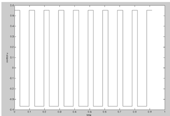
Fig. 6 Control input applied for achieving period 2. Control input is constant over a two successive impacts
