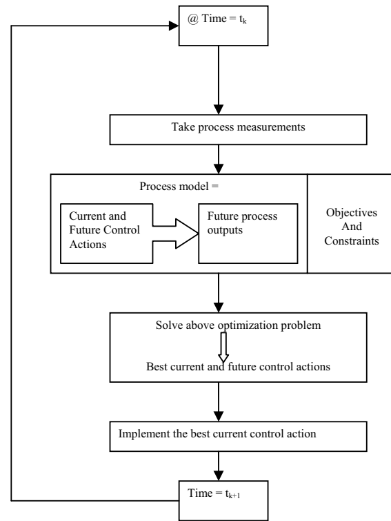
Fig. 3 Flowchart of Model Predictive Control
