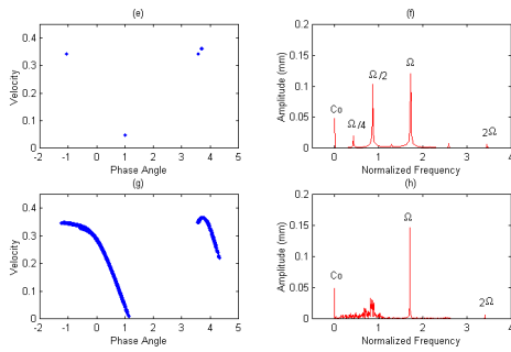
Fig. 3 Frequency spectra and Poincare maps of various responses of numerical simulations for A_0 = 3.0 V: (a) and (b) period-one motion, \Omega = 1.95 ; (c) and (d) period-two motion, \Omega = 1.80 ; (e) and (f) period-four motion, \Omega = 1.7255 ; (g) and (h) chaotic motion, \Omega = 1.708 .
