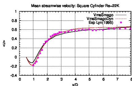
Fig. 7. Flow around a square cylinder at Reynolds 22000 : mean horizontal velocity on the centerline of the wake.
