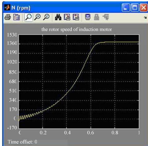
Fig. 8 Rotor speed of three-phase induction motor
