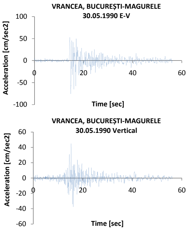
Fig. 7 Recorded accelererograms on N-S, E-V and vertical direction used in analysis from Vrancea earthquake, 30 May 1990, Bucharest-Măgurele
