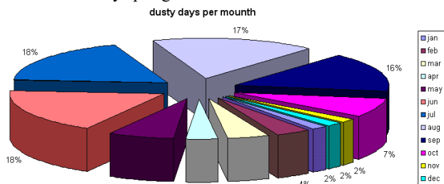
Fig. 10 Percentages of dusty days for different months over 1980-2005 period.
