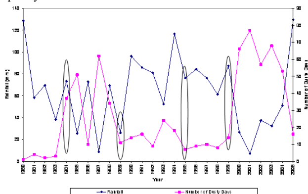
Fig. 8 Mean annual rainfall and number of dusty days (some abnormal cases identified by circles).
