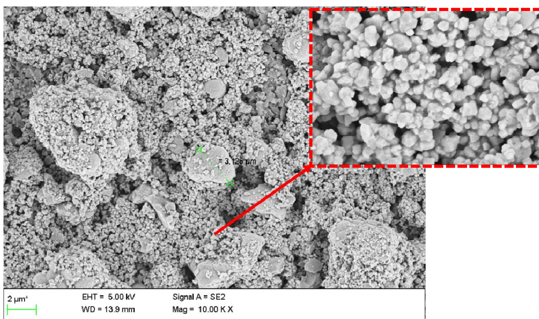
Fig. 2 Representative FESEM image of hierarchical superhydrophobic paper surface
