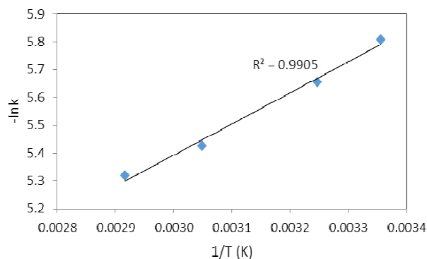
Fig. 6 Arrhenius plot for the dissolution rate
